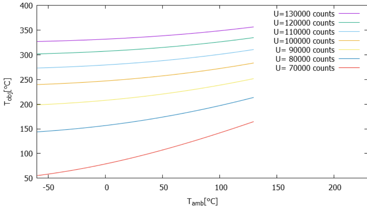
Figure 5: Typical temperature dependence of the raw thermopile output
