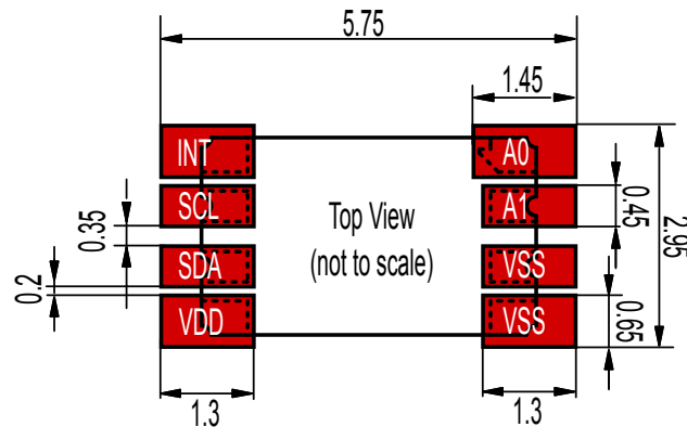
Figure 22: Recommended pad dimensions
