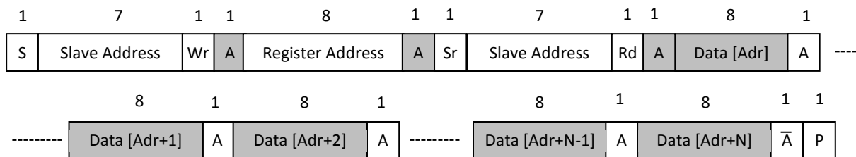
Figure 14: Reading EEPROM
