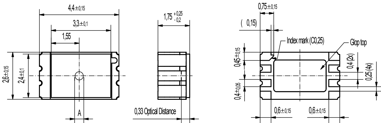
Figure 1: Mechanical Dimensions (in mm). The active pixel size diameter A is 0.5 mm.
