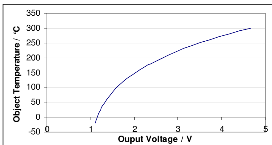
Figure 1: Output characteristic
